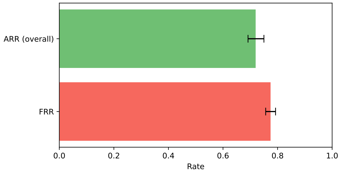
Overall ARR vs FRR (with 95% CI) (ARR↑ is good, FRR↓ is good)
