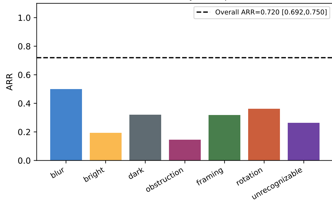
Actionable Recovery Rate per Defect
